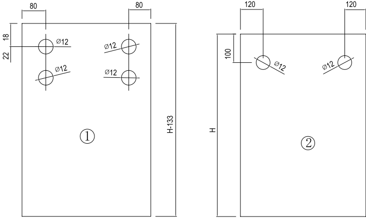
30X10方管截面安装图 Section Installation Diagram (30x10mm Square Tube)
