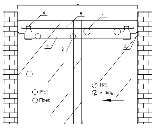
∅25管浴室吊轮平面安装图 Installation of ∅25 pipe bathroom hanging wheel
