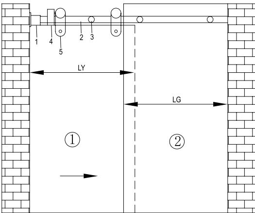
30X10方管平面安装图 Plane Installation Diagram (30x10mm Square Tube)
